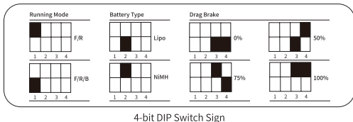
4-bit DIP Switch Sign
